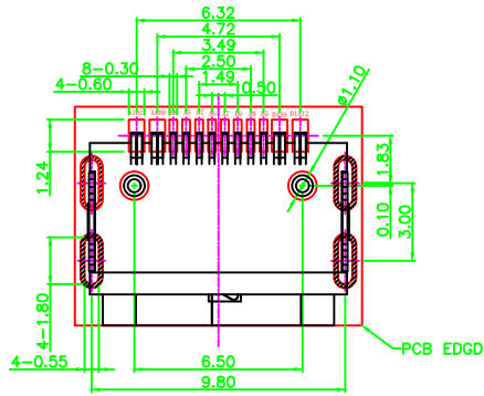
PCB LAYOUT TOLERANCESIZE:±0.05
