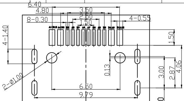
RECOMMENDED P.C.B. LAYOUT TOLERANCE UNSPECIFIED ±0.05mm
