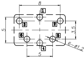
RECOMMENDED P. C. B. LAYOUT UNSPECIFIED TOLERANCE: \pm 0.05 (Copper-sided view)
