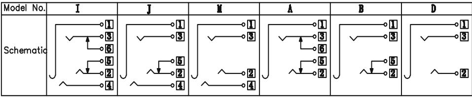
□: TERMINAL NO.
